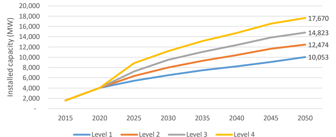
Installed capacity – Solar PV
